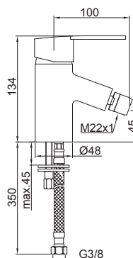
Monomando bidé con rótula giratoria, acabado cromo. Bidet single-lever mixer , directional aerator, chrome finish. Mitigeur bidet , bec orientable, fini chromé.
