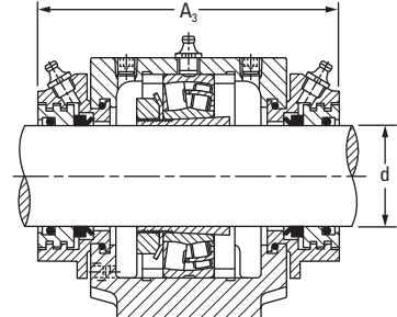
Taconite Seal
