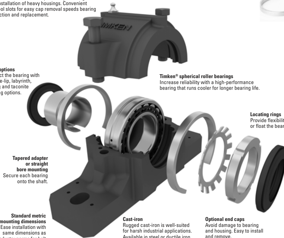
Fig. 25. SNT plummer block components and features.
