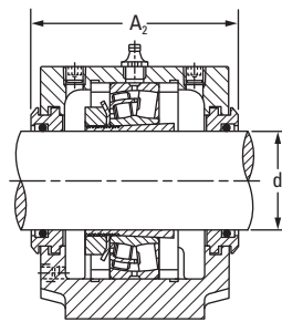
Labyrinth Seal
